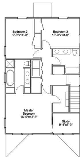
Second Floor 1,040 Sq. Ft. Clg. Ht. 9'
