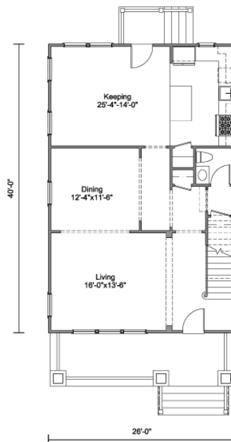
First Floor 1,040 Sq. Ft. Clg. Ht. 9'
